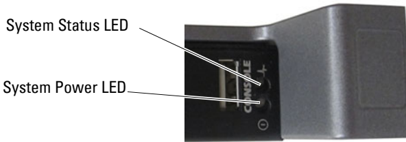
Figure 3-6. System LEDs
