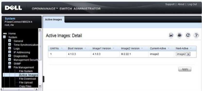
Figure 13-2. Active Images
