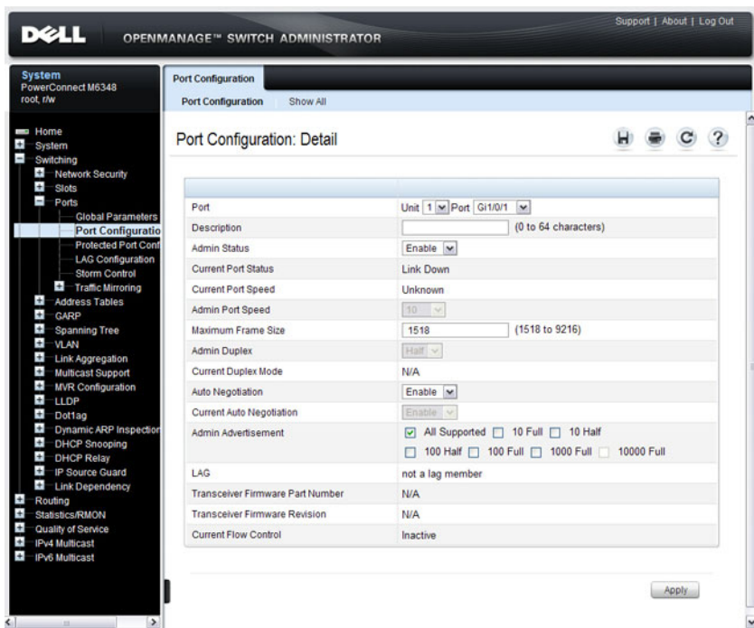
Figure 18-1. Port Configuration
