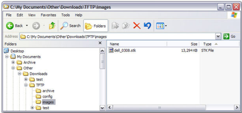
Figure 13-8. Image Path
