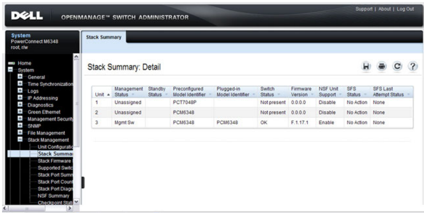
Figure 8-6. Stack Summary
