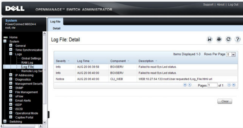
Figure 10-11. Log File
