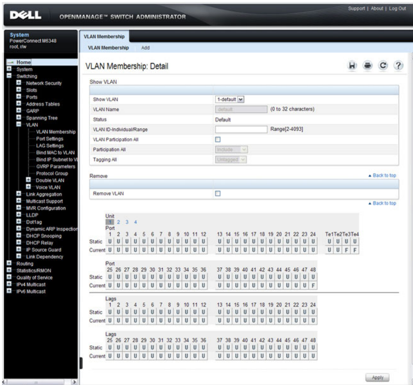
Figure 21-4. VLAN Membership
