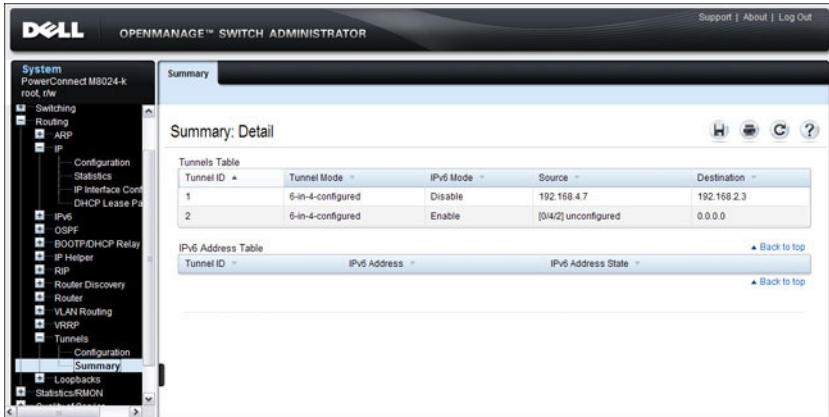
Figure 31-6. Tunnels Summary
