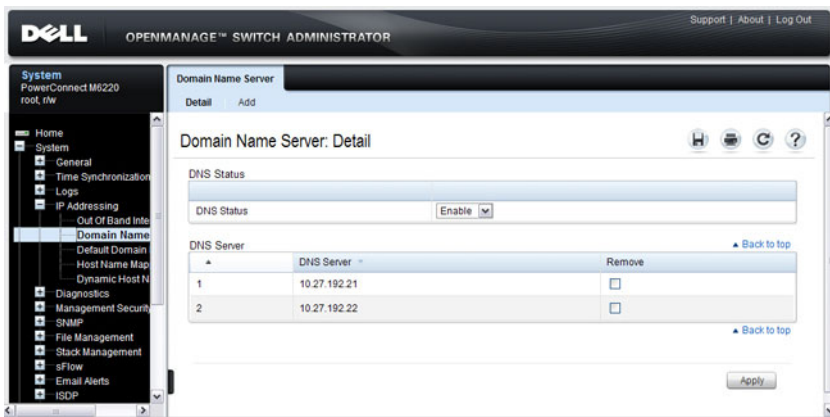
Figure 7-5. DNS Server
