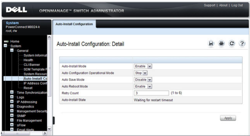
Figure 14-1. Auto-Install Configuration
