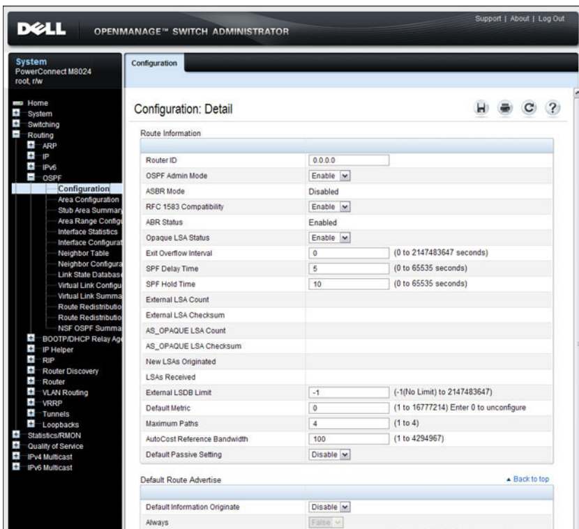
Figure 35-1. OSPF Configuration
