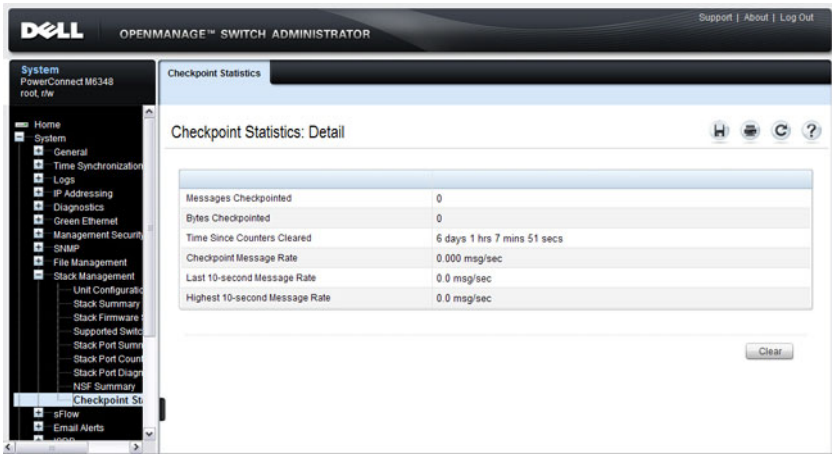
Figure 8-12. Checkpoint Statistics
