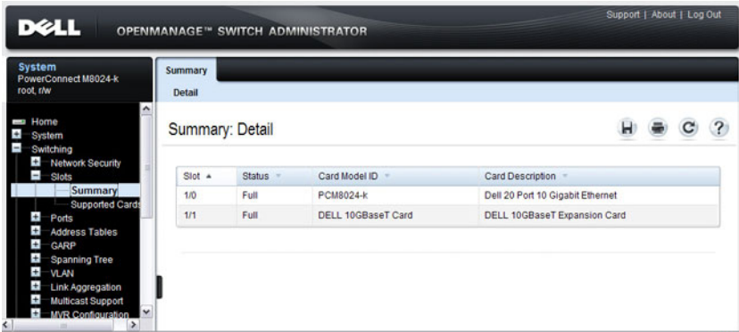
Figure 11-29. Slot Summary
