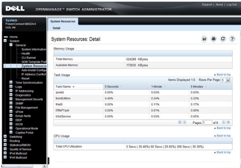
Figure 10-4. System Resources
