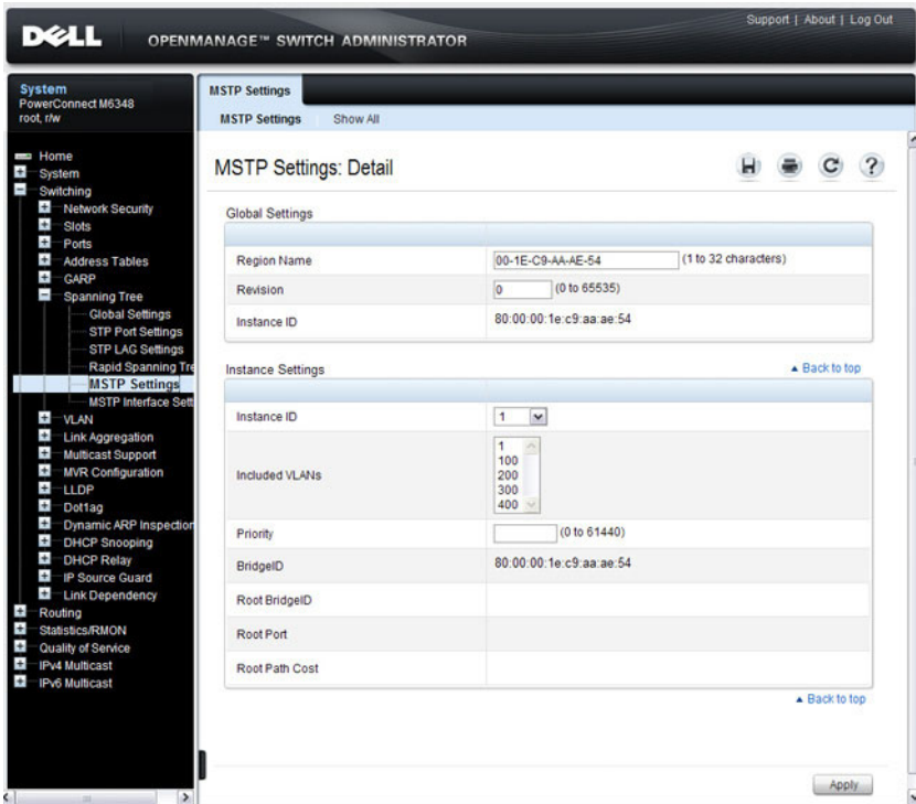
Figure 22-12. MSTP Settings
