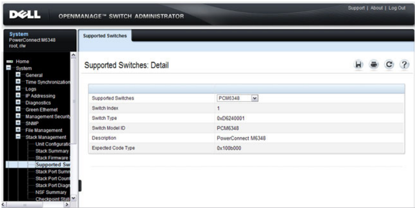
Figure 8-8. Supported Switches
