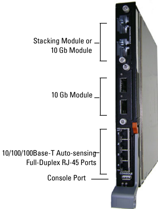
Figure 3-1. PowerConnect M6220 Front Panel
