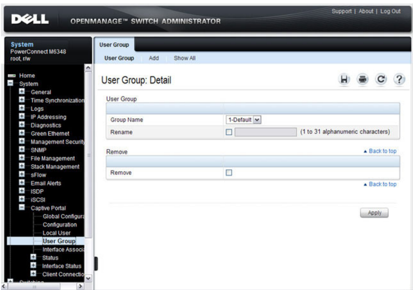
Figure 17-15. User Group
