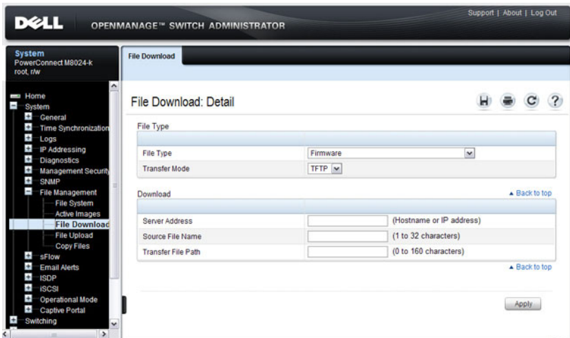
Figure 13-3. File Download
