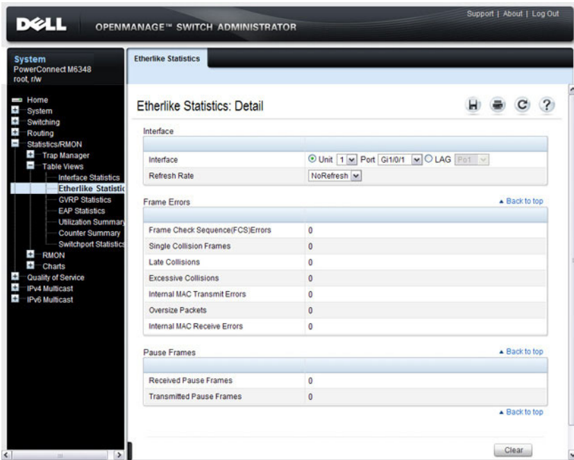
Figure 15-7. Etherlike Statistics
