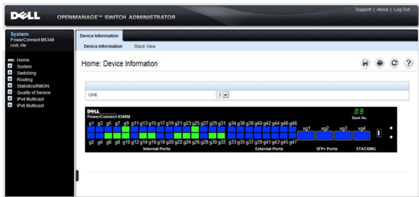
Figure 10-1. Device Information
