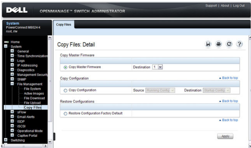
Figure 13-7. Copy Files
