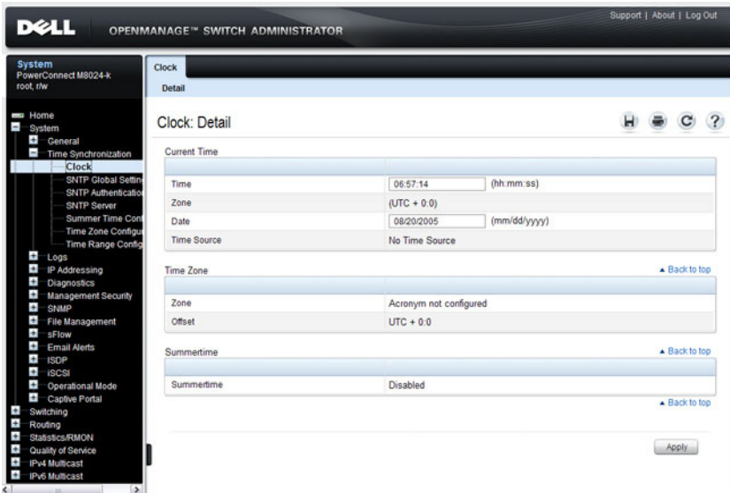
Figure 11-19. Clock
