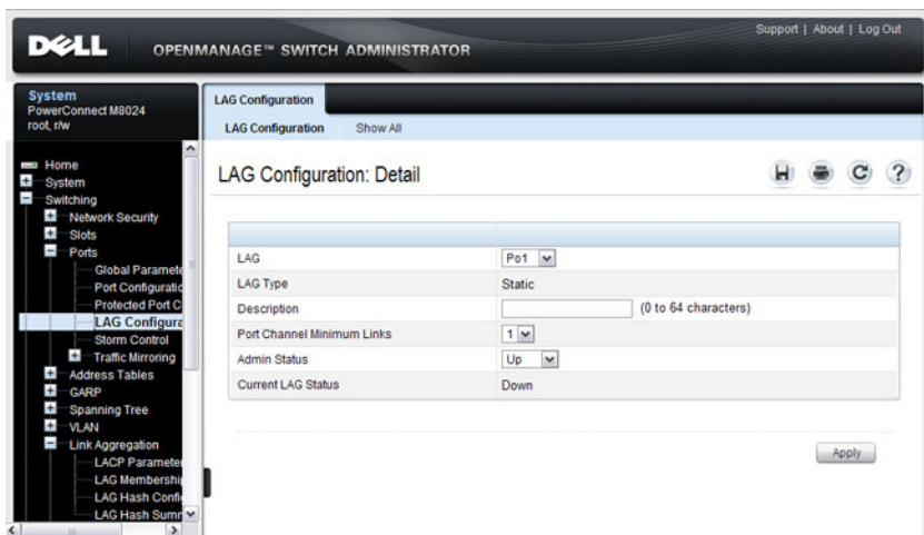
Figure 28-2. LAG Configuration
