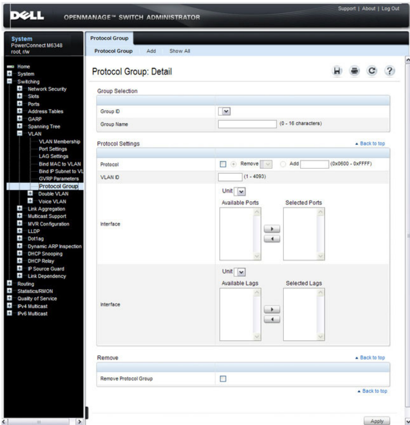
Figure 21-18. Protocol Group
