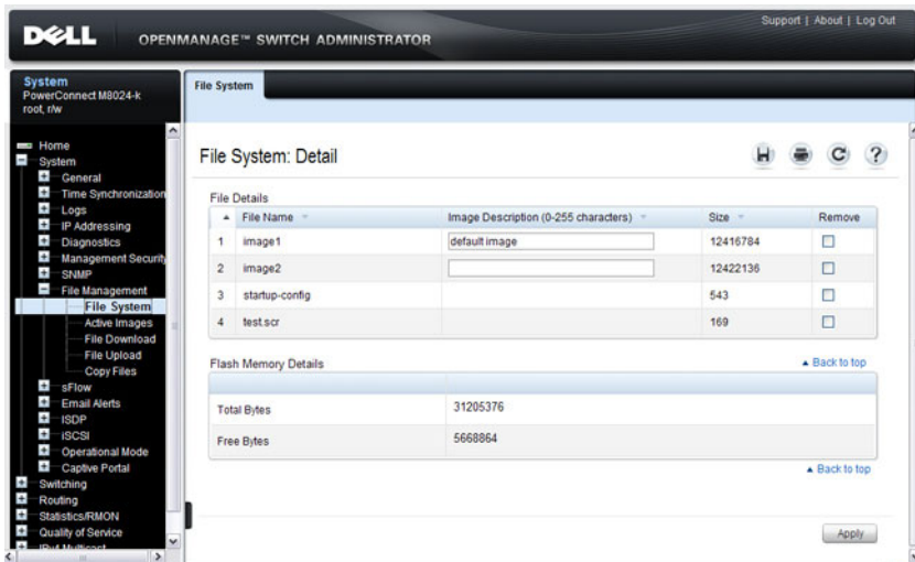
Figure 13-1. File System
