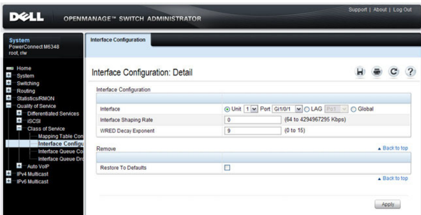
Figure 41-3. Interface Configuration
