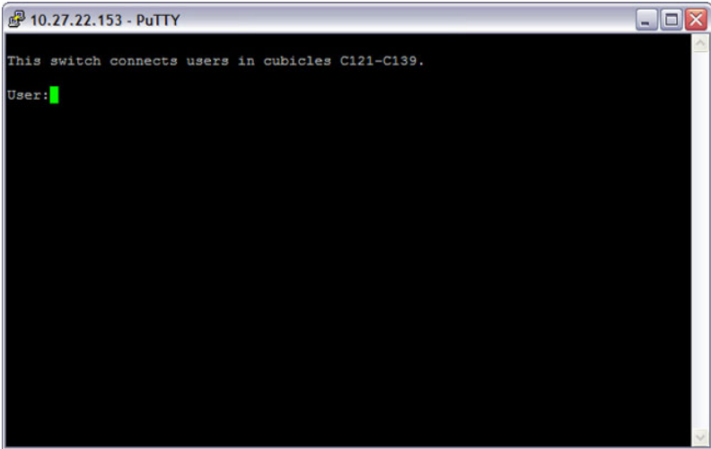
Figure 11-31. Verify MOTD
