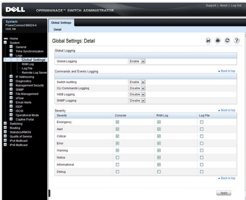
Figure 10-9. Global Settings
