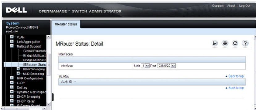
Figure 25-4. MRouter Status
