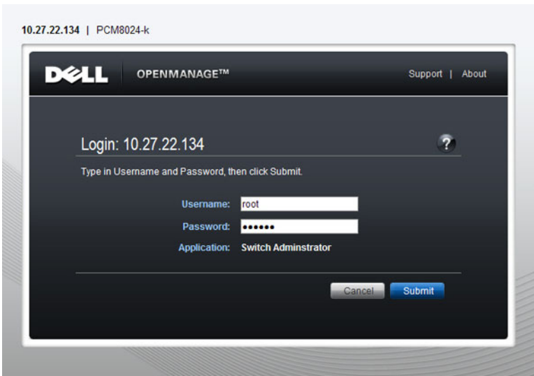
Figure 4-1. Login Screen
