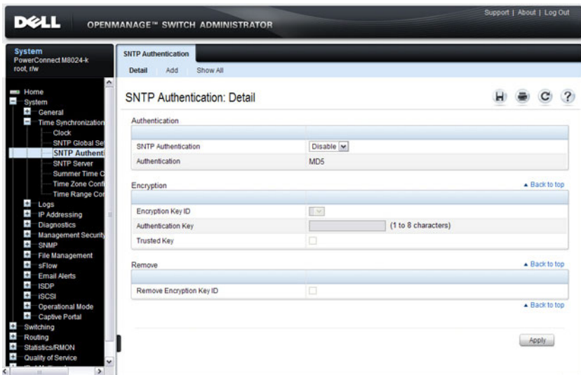
Figure 11-21. SNTP Authentication
