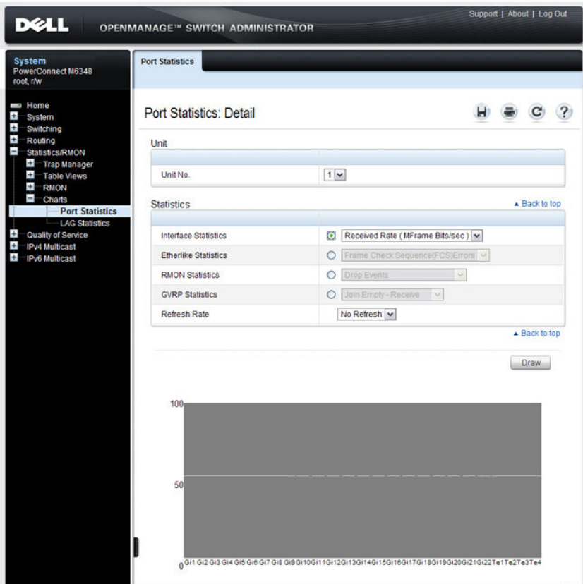
Figure 15-22. Ports Statistics
