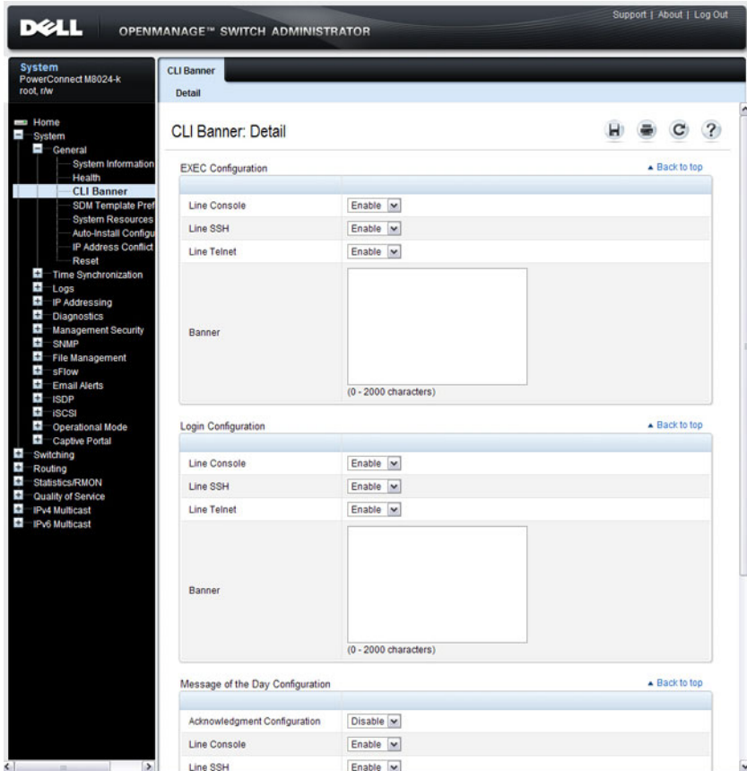
Figure 11-5. CLI Banner
