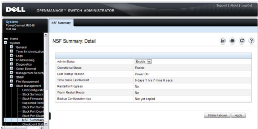
Figure 8-11. NSF Summary
