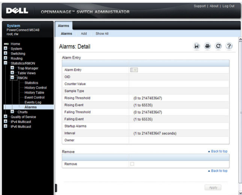
Figure 15-20. RMON Alarms
