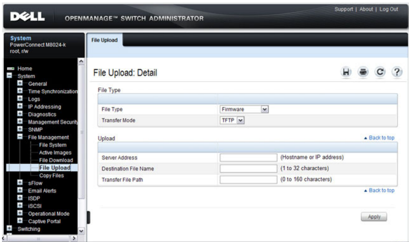
Figure 13-5. File Upload
