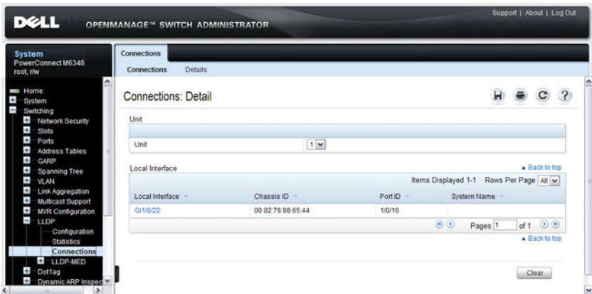
Figure 23-9. LLDP Connections
