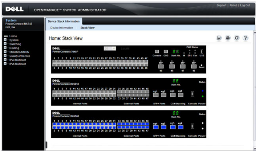
Figure 10-2. Stack View
