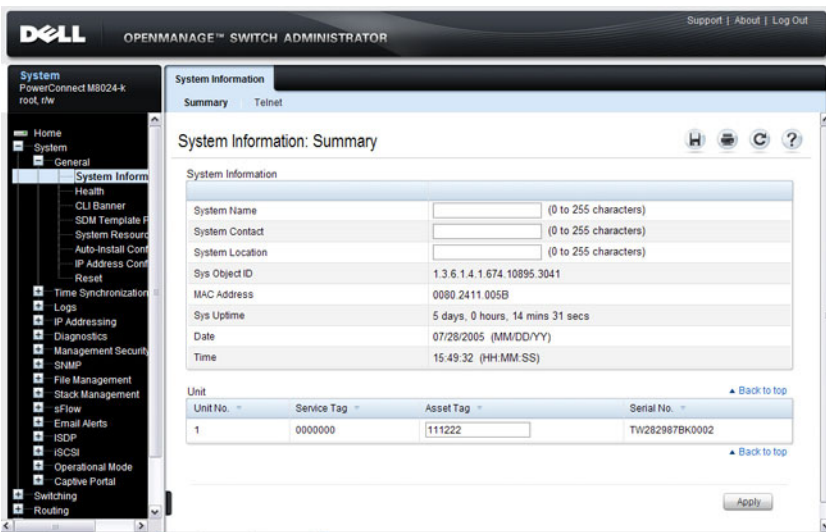
Figure 11-1. System Information
