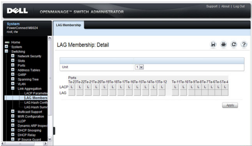
Figure 28-5. LAG Membership
