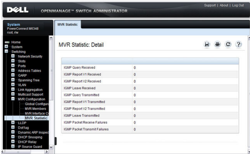
Figure 25-29. MVR Statistics
