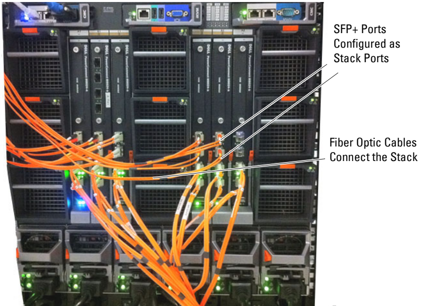
Figure 8-3. Connecting a Stack of PowerConnect M8024-k Switches
