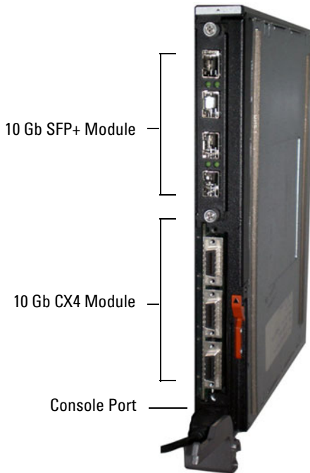
Figure 3-3. PowerConnect M8024 Front Panel
