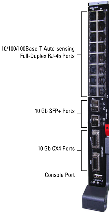
Figure 3-2. PowerConnect M6348 Front Panel
